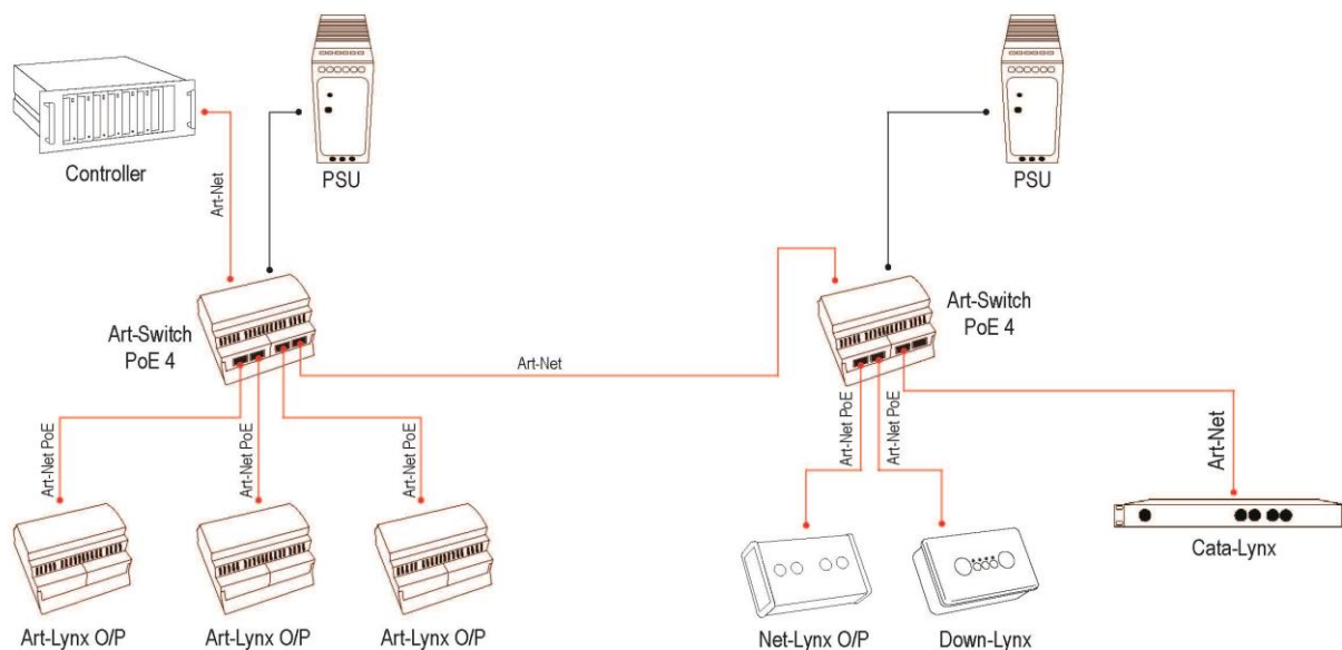
Wiring Drawing
